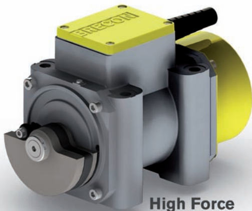
The two-step concrete compaction with Brecon 2in1 vibrators is advantageous at a high percentage of reinforcement.
